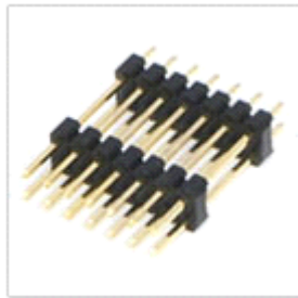
PLDD Series 2 Row 2 lines, Straight 2.00 / 2.54mm
