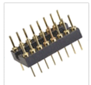
SCSL Series IC Socket, Round Pins 2.54mm
