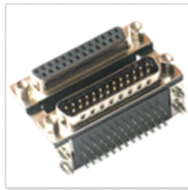
DR25F/25M Right Angle Type 25F / 25M
