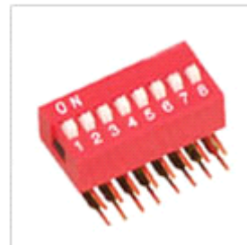
DA3 Series DIP Switch Special R/A (90°) Type
