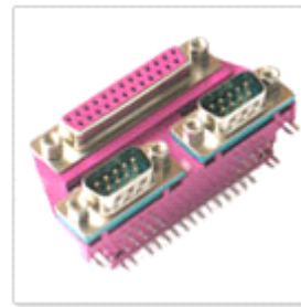
DR25F/9M/9M Right Angle Type 25F / 9M / 9M
