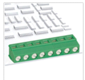
GS009R Pitch: 5.00 / 5.08mm 300V/12A 1.5MM 2
